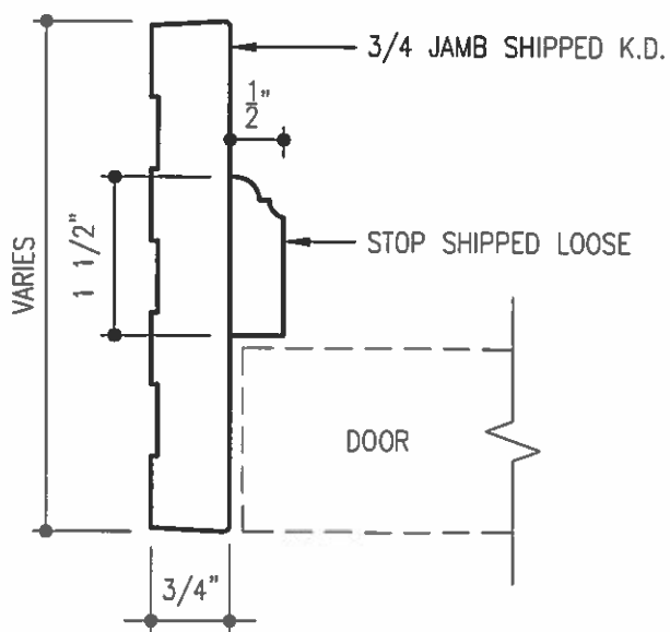
3/4 INTERIOR JAMB COLONIAL STOP
