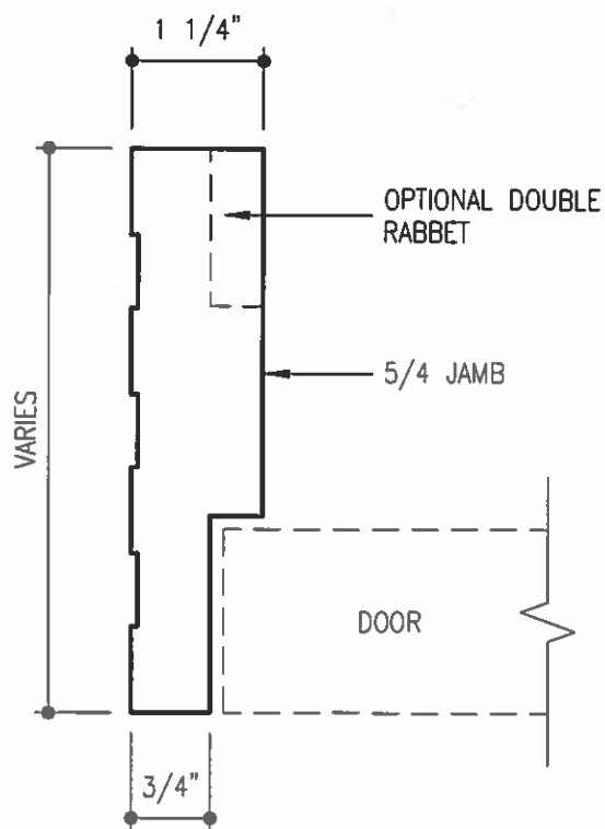
5/4 RABBETED JAMB
