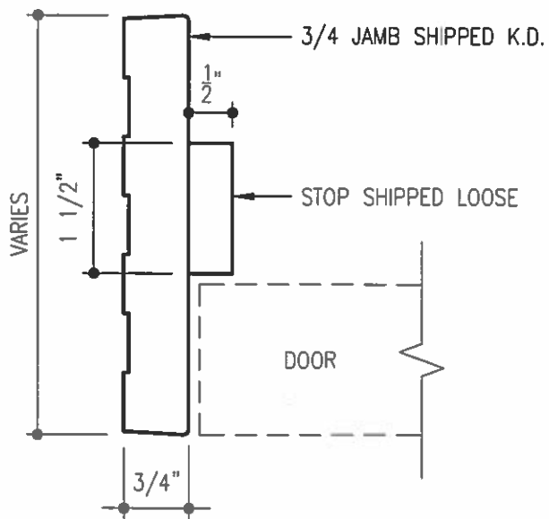
3/4 INTERIOR JAMB RECTANGULAR STOP
