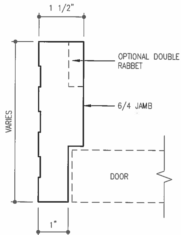
6/4 RABBETED JAMB
