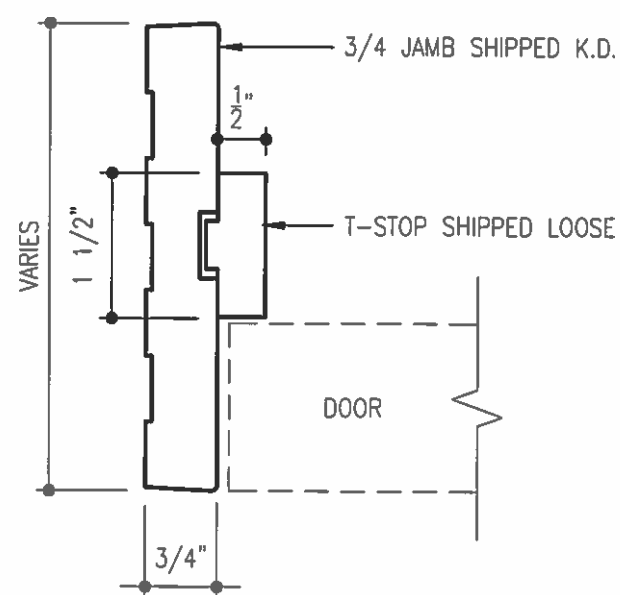
3/4 INTERIOR JAMB T-STOP
