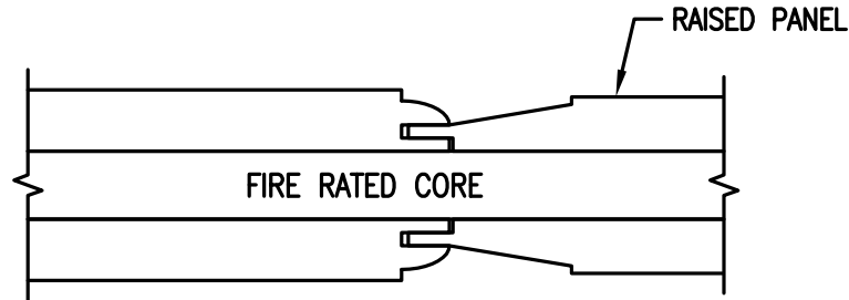
STANDARD PROFILE – PANEL A1
