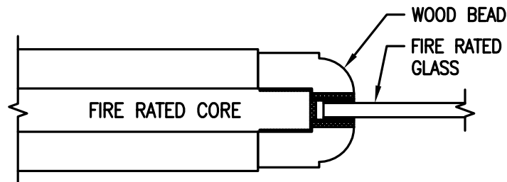
STANDARD PROFILE – WOOD BEAD
