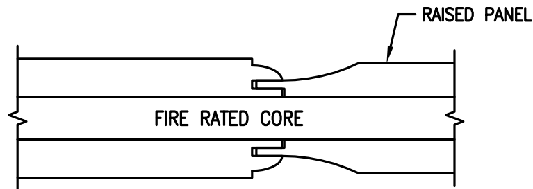
STANDARD PROFILE – PANEL 2
