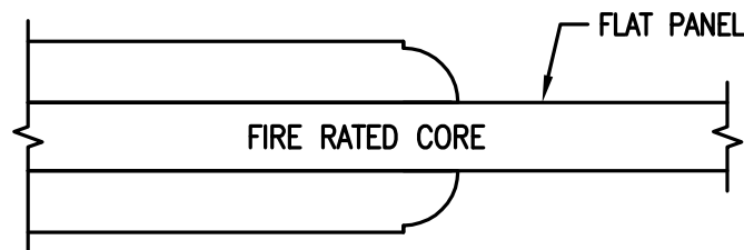
STANDARD PROFILE – FLAT PANEL
