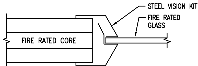
STANDARD PROFILE – VISION KIT
